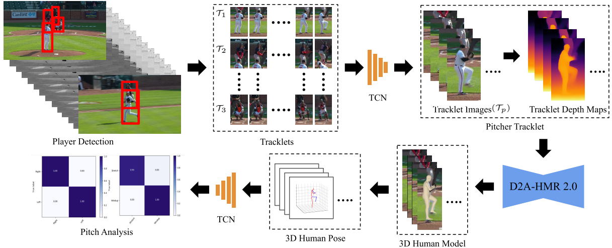
Figure 6.2: Overall architecture. Given a video broadcast, we begin by extracting player tracklets, denoted as \mathcal{T} \in \{\mathcal{T}_1, \mathcal{T}_2, \dots, \mathcal{T}_n\} . Each tracklet \mathcal{T}_k consists of a sequence of frames \mathbf{F}_i where \mathbf{F}_i \in \mathbb{R}^{H \times W \times 3} for N frames. These tracklets are then processed through a TCN, which implicitly decouples player actions and identifies the tracklet of the pitcher, called \mathcal{T}_p . Subsequently, \mathcal{T}_p undergoes encoding via an encoder ( E ) to derive pseudo-depth information for each frame. The frames, along with their corresponding pseudo-depth data, are fed into a 3D modeling technique ( D2A-HMR 2.0 ). This framework is responsible for predicting the 3D mesh and 3D joint positions of the pitcher, facilitating detailed analysis of various pitch metrics using the temporal kinematic information processing the 3D joint positions.
