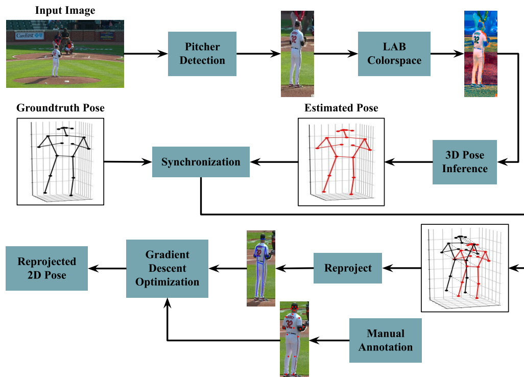
Figure 3.2: Overview of the data processing framework.
