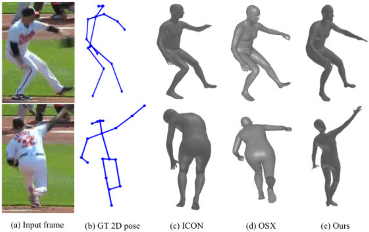
Figure 4.3: Qualitative evaluation of 3D human model in handling motion blur effects.
