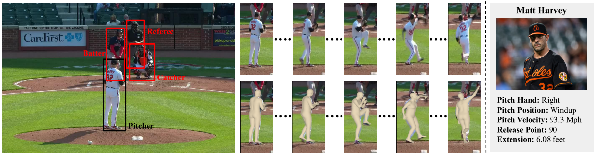
Figure 6.1: 3D player reconstruction and kinematic-driven pitch statistics from monocular video. We introduce PitcherNet , a pioneering deep learning system that tackles low-resolution video limitations through efficient 3D human modeling for robust player alignment (left) and reliable pitch statistics analysis from estimated kinematic data (right).
