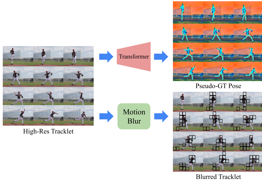
Figure 6.3: Data Augmentation Technique. Pseudo-ground truth pose is collected using a Transformer model for improved generalizability of the pose estimation model.
