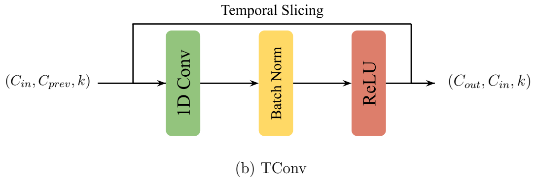
Figure 3.3: Temporal Convolutional Network. (a) Overview of the proposed TCN for the player identification task, where fc denotes fully connected layers and p refers to the model's output. (b) Architecture of the TConv block used in the TCN, where C_{in} , C_{out} and C_{prev} denotes the input, output and previous channels, respectively and k denotes the kernel size.
