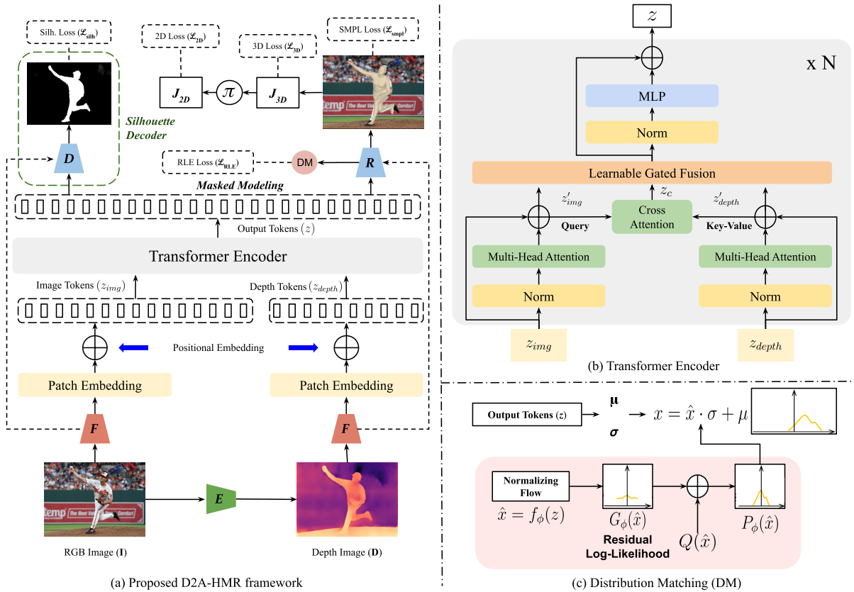
Figure 5.1: Overview of the D2A-HMR model architecture. Given an image ( \mathbf{I} ), we first incorporate a transformer backbone ( \mathbf{E} ) to estimate the depth map ( \mathbf{D} ) and a CNN backbone ( \mathbf{F} ) to extract the features from the images. Positional embedding is applied to both image and pseudo-depth features, utilizing a hybrid approach for image tokens ( z_{img} ) and a learnable position embedding for pseudo-depth tokens ( z_{depth} ). Self-attention is performed on z_{img} and z_{depth} , resulting in z'_{img} and z'_{depth} , respectively. Subsequently, cross-attention is applied between z'_{img} and z'_{depth} to produce z_c . The learnable fusion gates combine z'_{img} , z'_{depth} , and z_c , followed by layer normalization and a Multi-Layer Perceptron (MLP). The resulting gated tokens ( z ) are input into two distinct refinement modules: a decoder ( \mathbf{D} ) for silhouette estimation and a regressor head, \mathbf{R} which incorporates normalizing flow ( \mathbf{DM} ) for distribution-aware joint vertex estimation.
