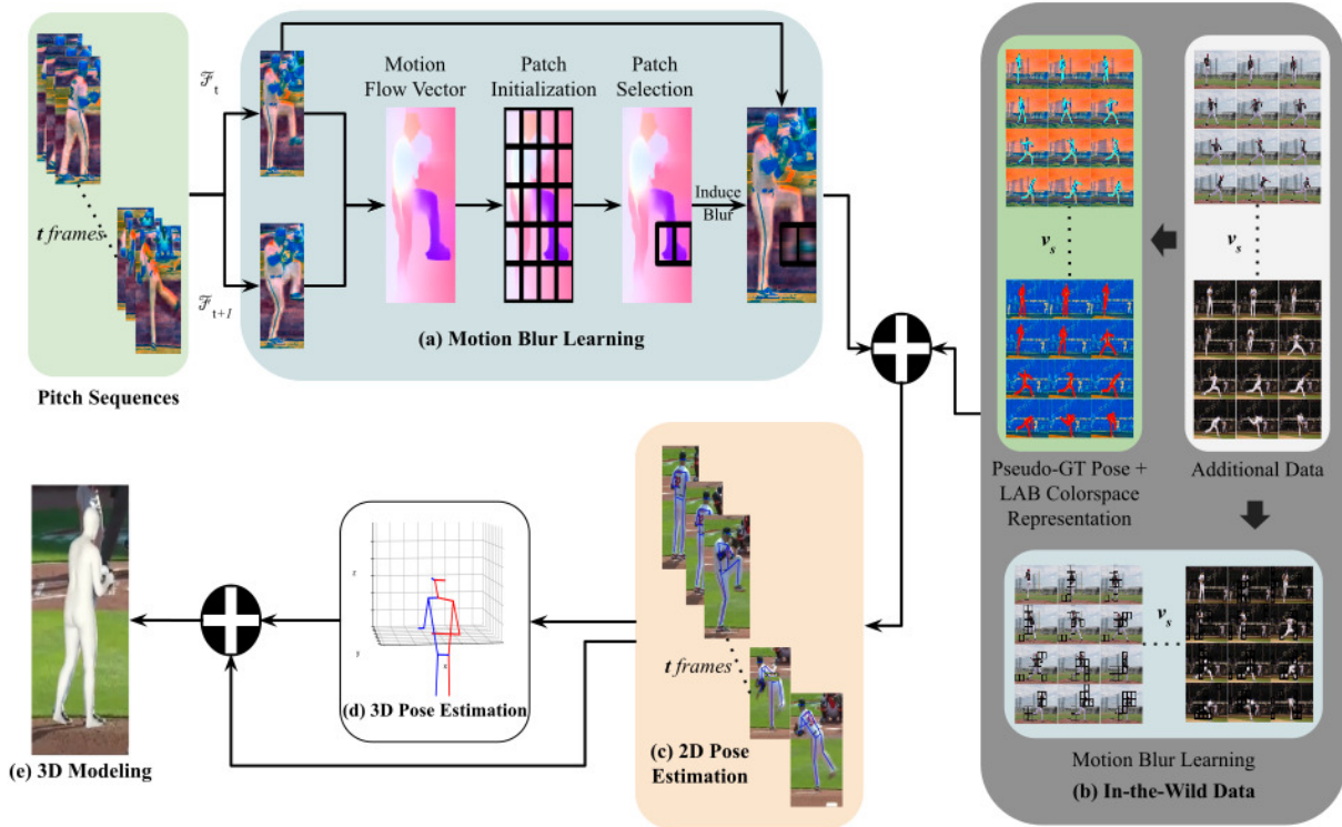
Figure 4.2: Overview of the proposed system. (a) The motion blur learning module creates synthetic blur effects on the pitch sequences to learn better features and generalize well despite such effects. (b) In-the-wild data is leveraged to enhance the robustness of the model on diverse environmental conditions. (c) A regressor-based 2D pose estimator to train the data from the motion blur learning module and the in-the-wild data. (d) A transformer-based 3D pose estimator to train on sequential 2D pose data to estimate the 3D pose. (e) Concatenation of the 2D and 3D poses to estimate the 3D body mesh using spectral GCN.
