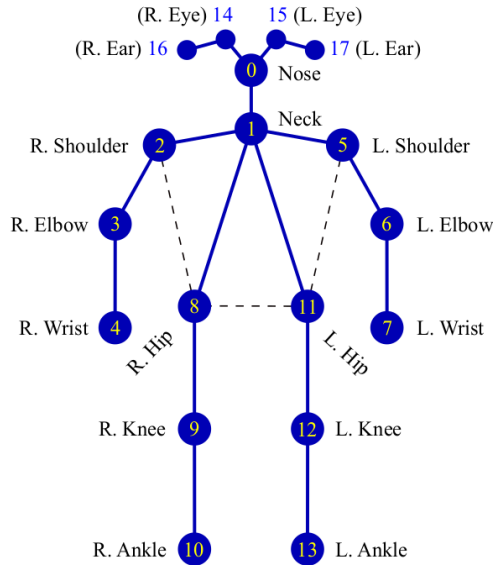
Figure 3.1: Ground truth format for the 3D joint positions (R/L: right/left).
